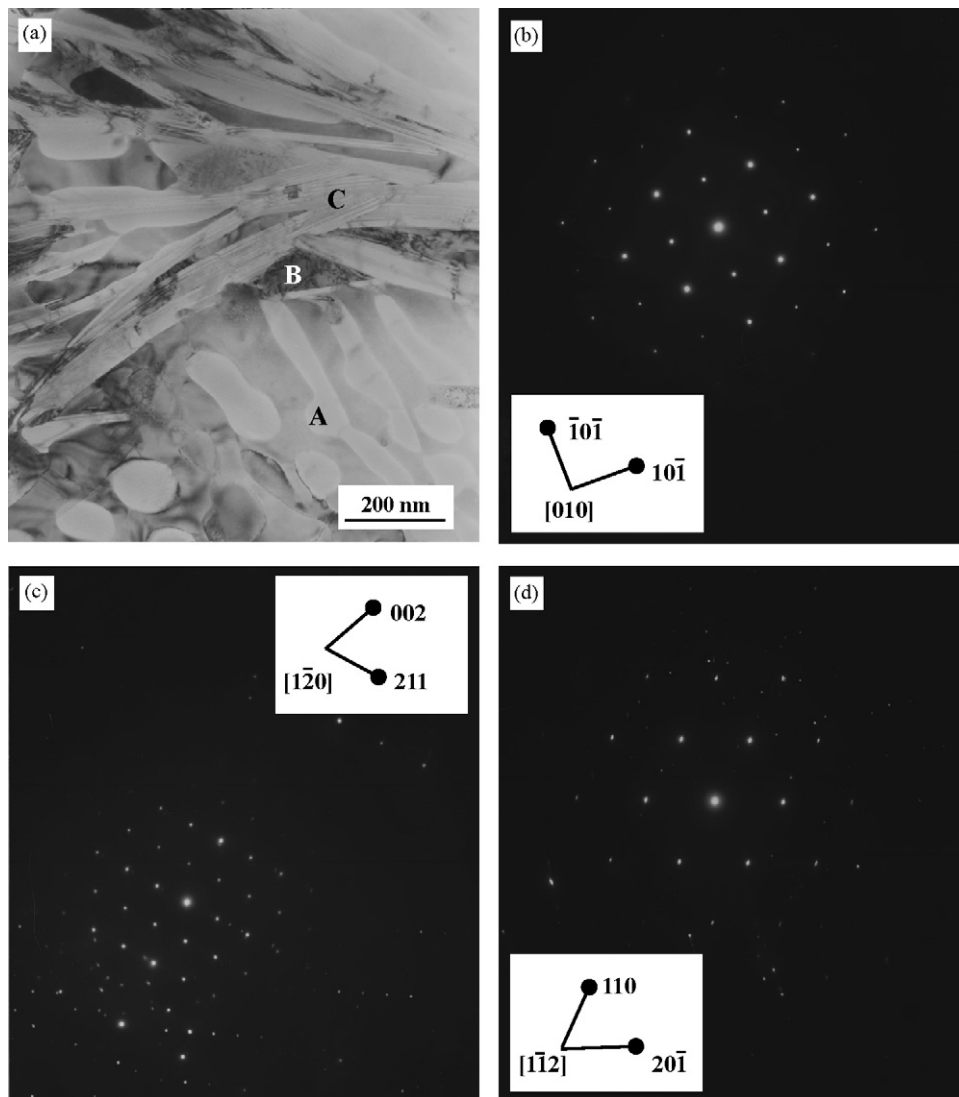
Fig. 3. TEM images showing the eutectic microstructure with elongated and striated bands (a) and SAED patterns corresponding to site A (b), site B (c) and site C (d) in (a) of as-cast \text{Cu}_{52.5}\text{Ti}_{30}\text{Zr}_{11.5}\text{Ni}_6 sample with 6 mm diameter.
