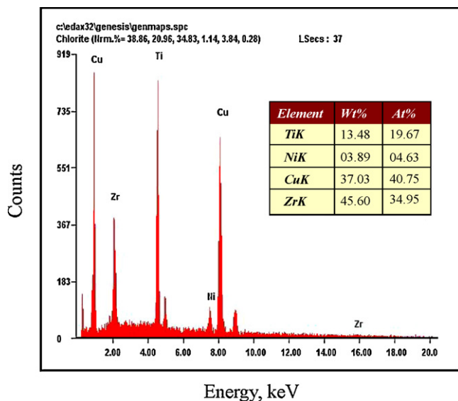
Fig. 4. EDX spectrum showing the element contents of a detected CuZr particle.
