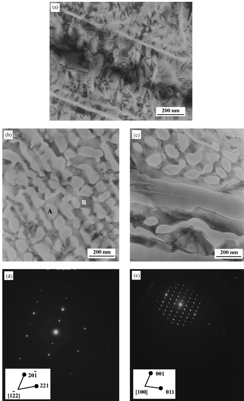
Fig. 2. TEM images showing the decomposition of amorphous matrix (a), eutectic microstructure with lamellar configuration (b) and (c), and SAED patterns corresponding to sites A (d) and B (e) in (b) of as-cast \text{Cu}_{52.5}\text{Ti}_{30}\text{Zr}_{11.5}\text{Ni}_6 sample with 6 mm diameter.
